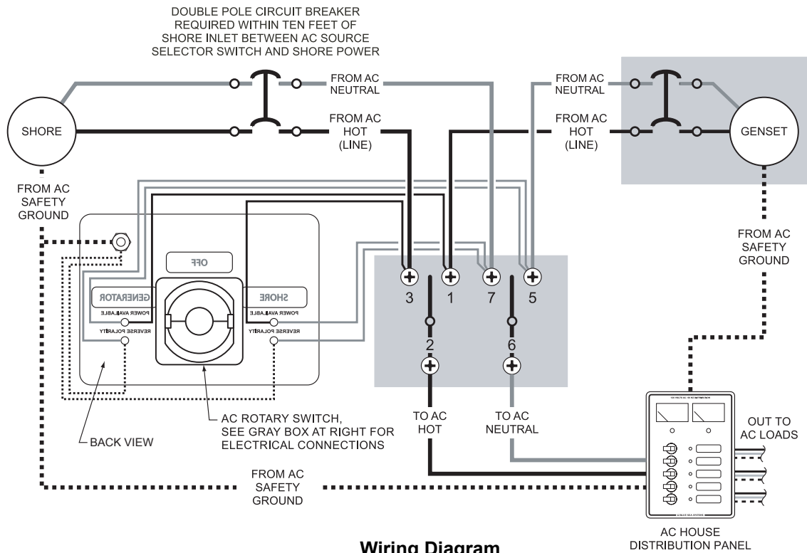
Wiring Diagram AC Source Selector Panel PN 8367 Shown
